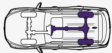
2WD high range
