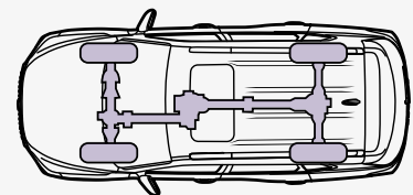
4WD low range
